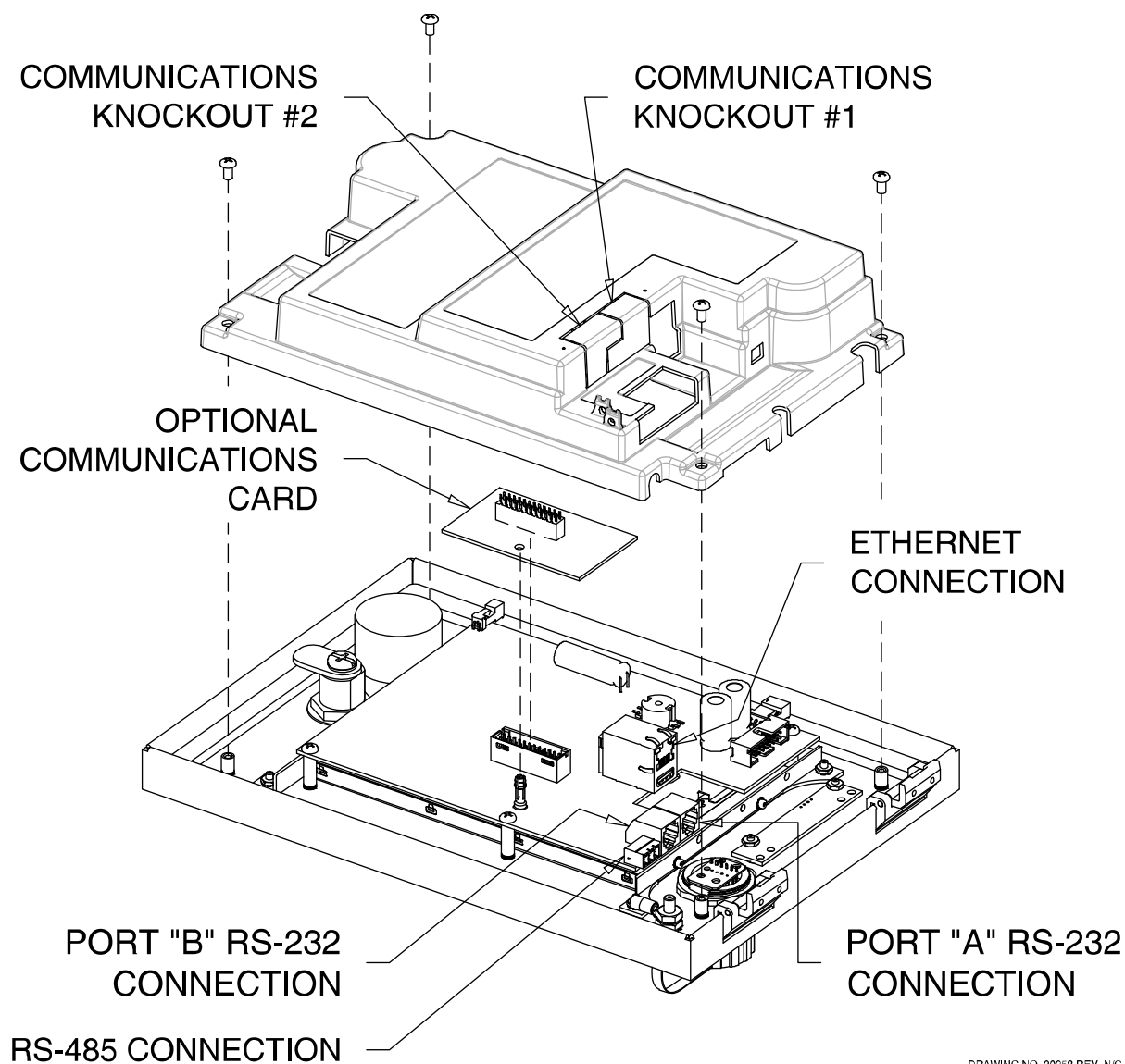
Figure 3-11 - Non-Hazardous Expansion Option Installation – Processor Board
