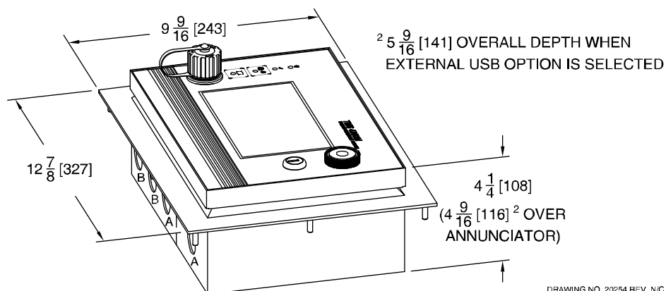
Figure 1-2 - TMS4000M Console Outline
