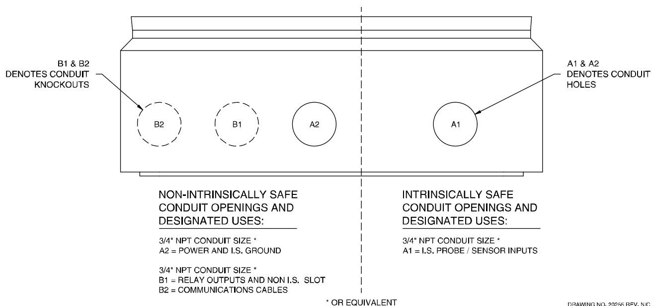
Figure 1-3 - TMS4000M Designated Conduit Locations
