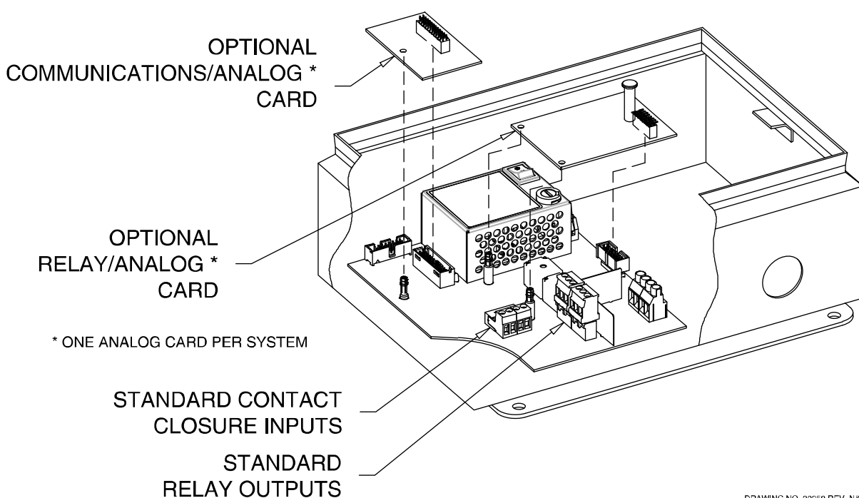
Figure 3-10 - Non-Hazardous Expansion Option Installation – Main Board
