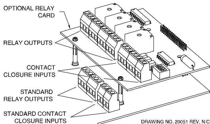
Figure 3-7 - Relay Output/Contact Closure Input Layout (Optional 4 Relay Output/4 Contact Closure Input Expansion Card shown)
