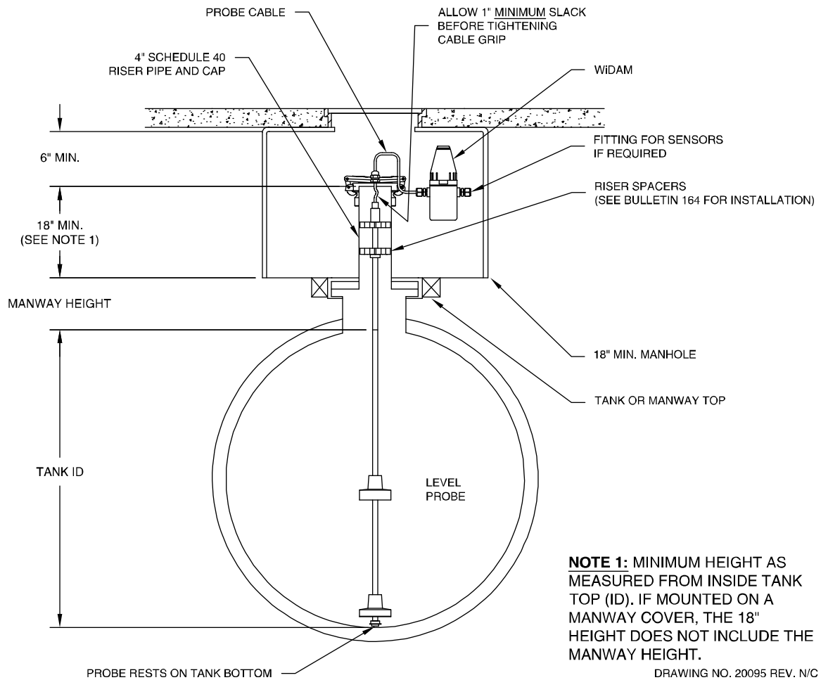
Figure 2-3 - Level Probe Installation - Underground Tank
