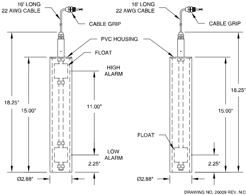
Figure 1-9 – RSU800
