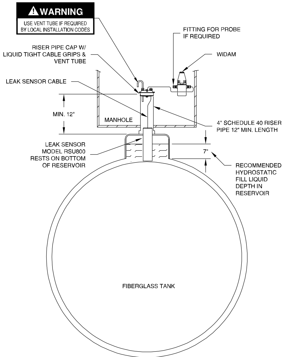
Figure 2-11 - Hydrostatic Leak Sensor Installation in Fiberglass Tanks
