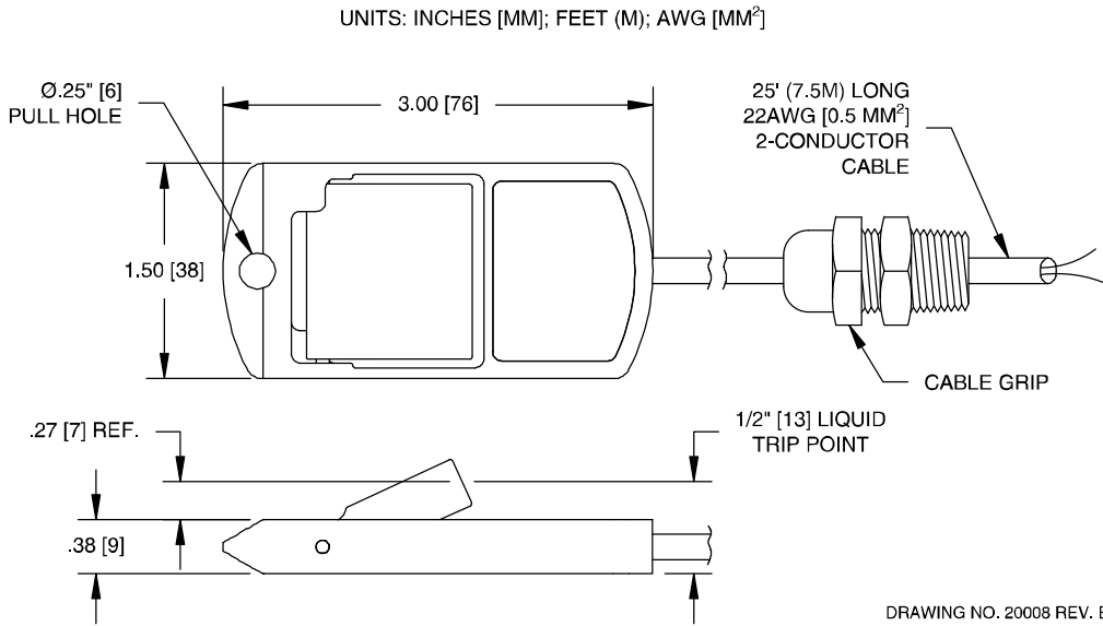
Figure 1-8 – LS610
