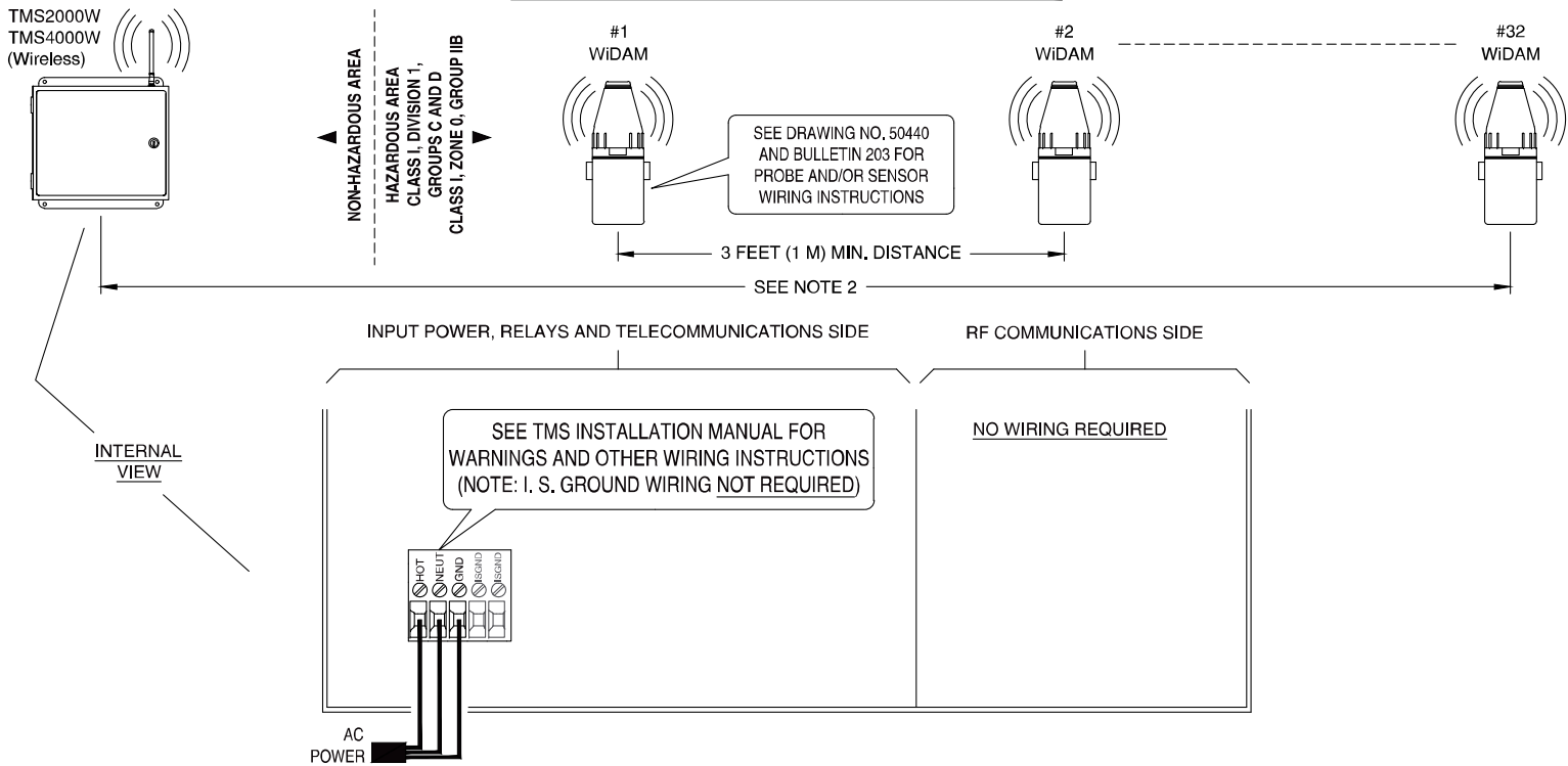
Figure 3-1-1 - TMS2000W1 AC Power Wiring
