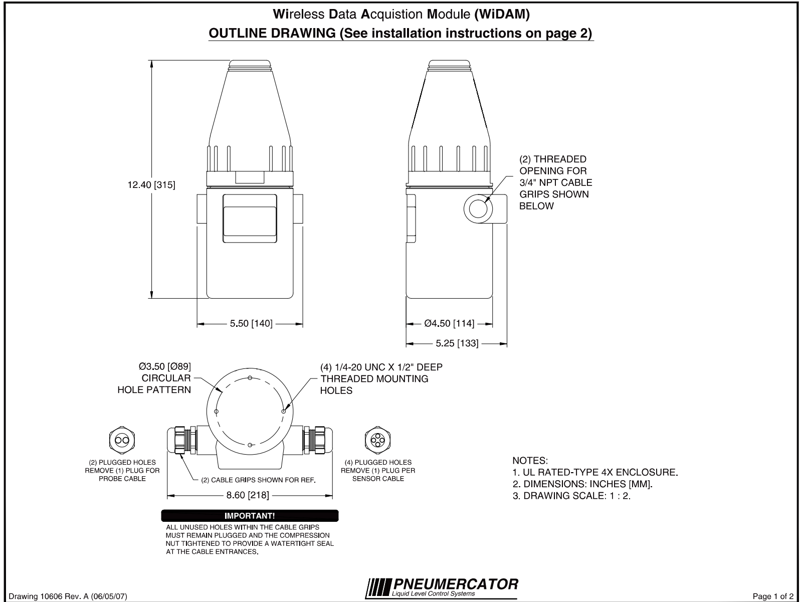
Figure 1-4 – WiDAM Overview
