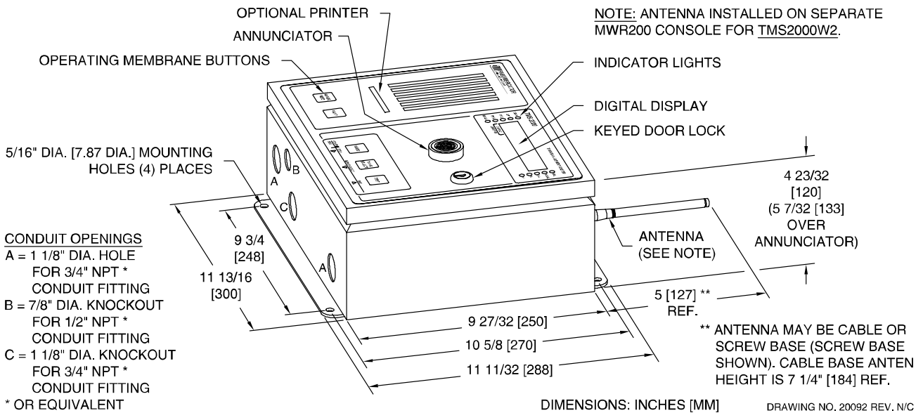
Figure 1-2 - TMS2000 Console Outline
