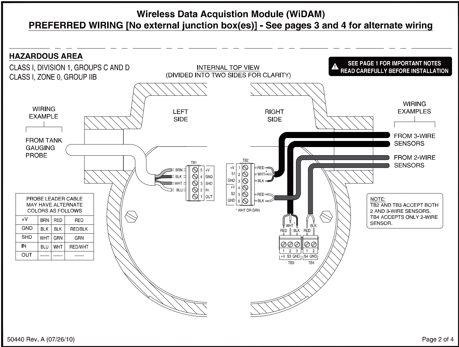
Figure 3-2-2 - Preferred Wiring
