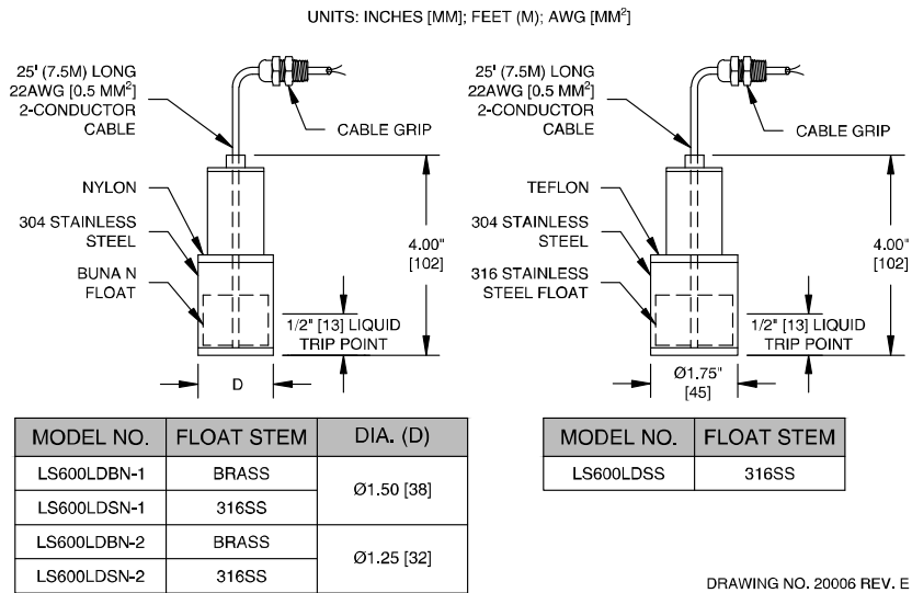
Figure 1-6 – LS600 LD Series
