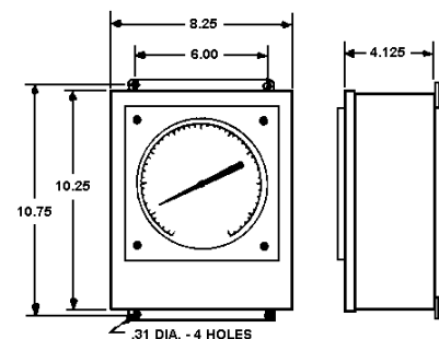
INDICATOR DETAIL
